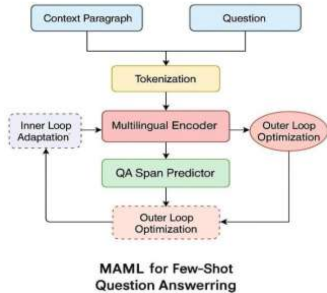
Fig. 2. AML-based framework for adapting QA models to new languages using few-shot question-answer pairs
