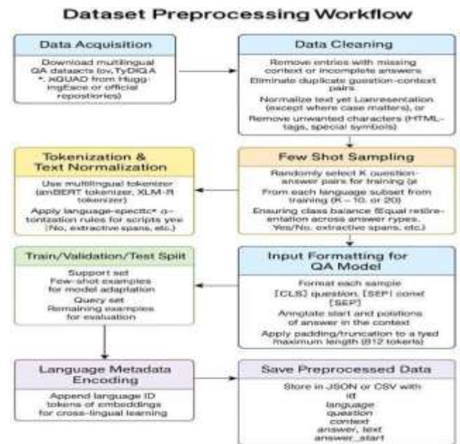
Fig. 1. Workflow for preprocessing multilingual QA datasets (TyDiQA, XQuAD) for few-shot learning in low-resource languages.
